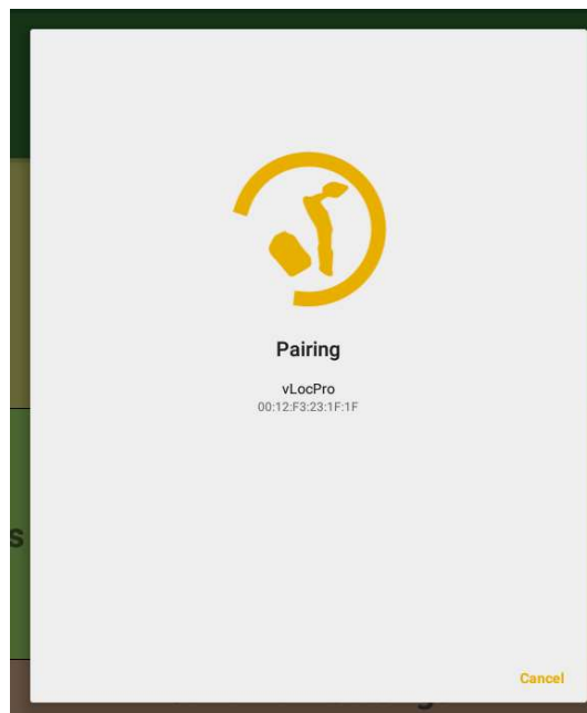
Figure 30 - Pairing message
