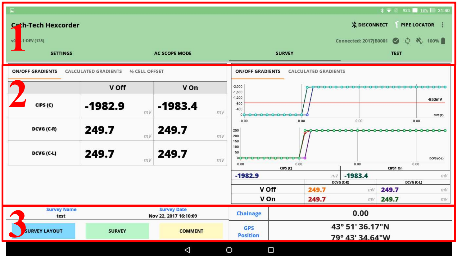
Figure 20 - Survey Screen
