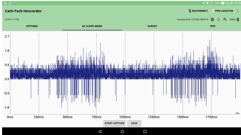
Figure 24 - AC Scope Screen
