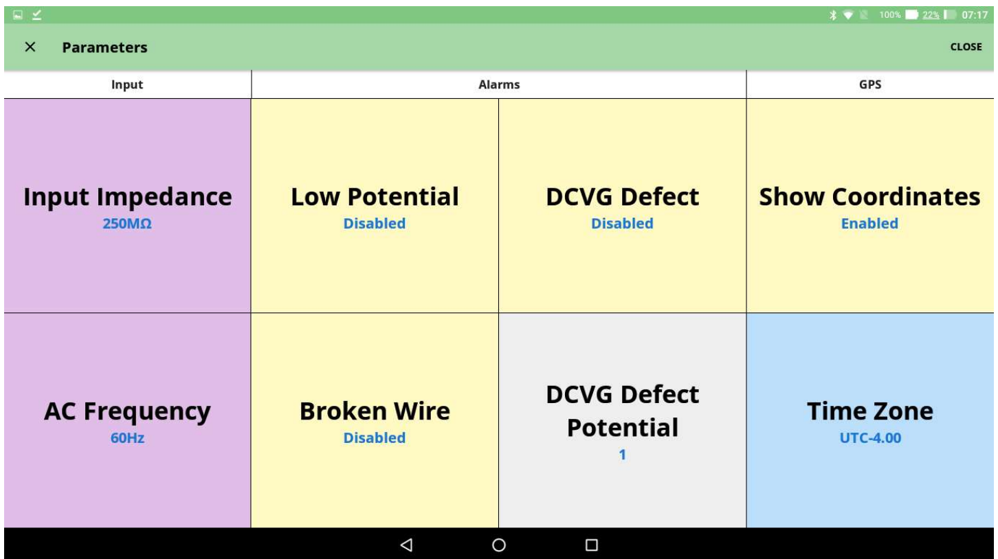
Figure 12 - Parameters Screen
