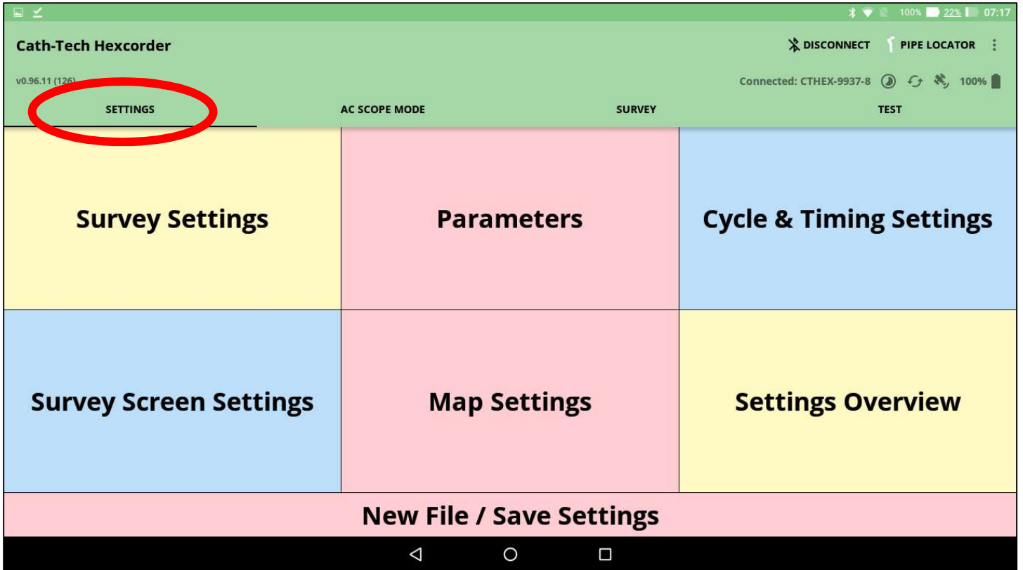
Figure 10 - Settings Tab
