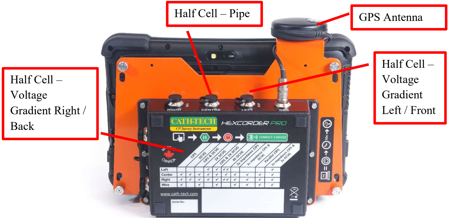
Figure 4 - Hexcorder Pro assembly - Bottom view
